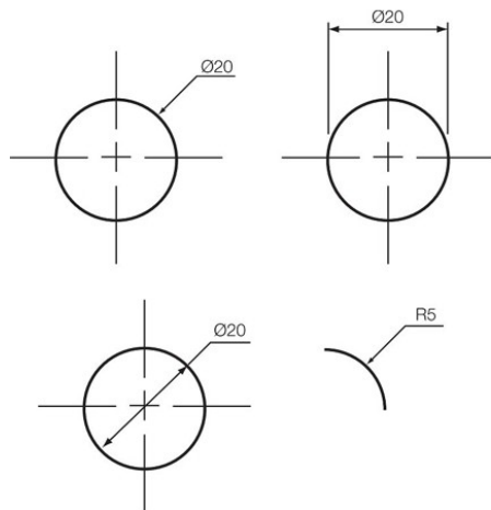
▲ Dimensioning circles.
