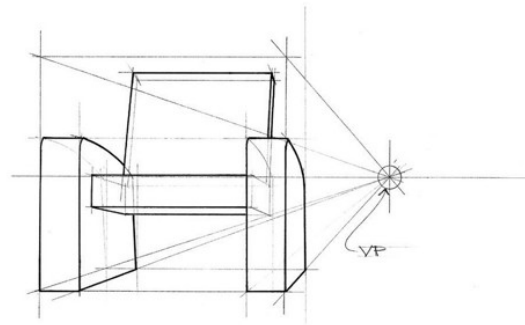
▲ One-point perspective drawing of club armchair using crating method
