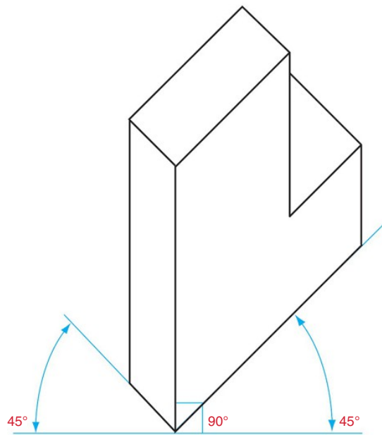
▲ Planometric drawing
