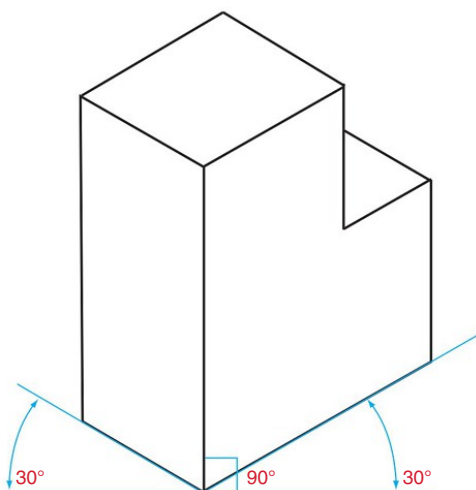
▲ Isometric drawing
