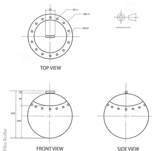
▲ Orthogonal drawing of a handbag design.
