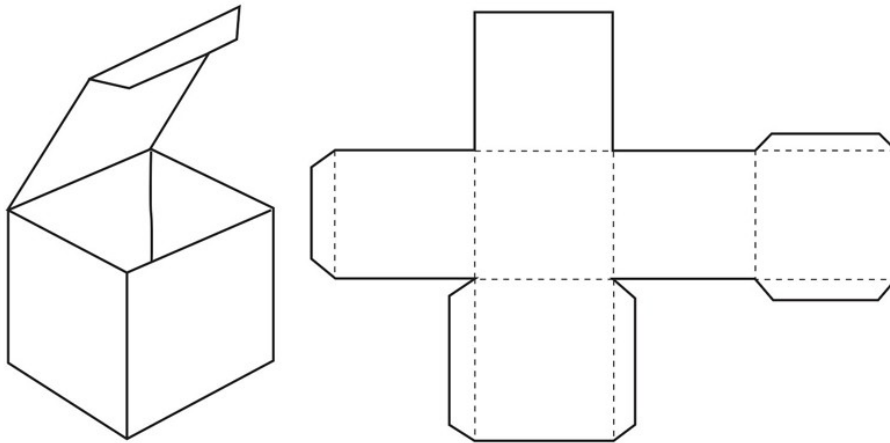
▲ Packaging net of a simple box
