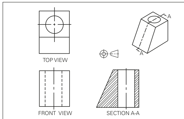
Figure 4.23 Third-angle orthographic drawing with the side view in section
