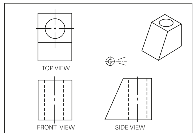
Figure 4.18 Centre line
