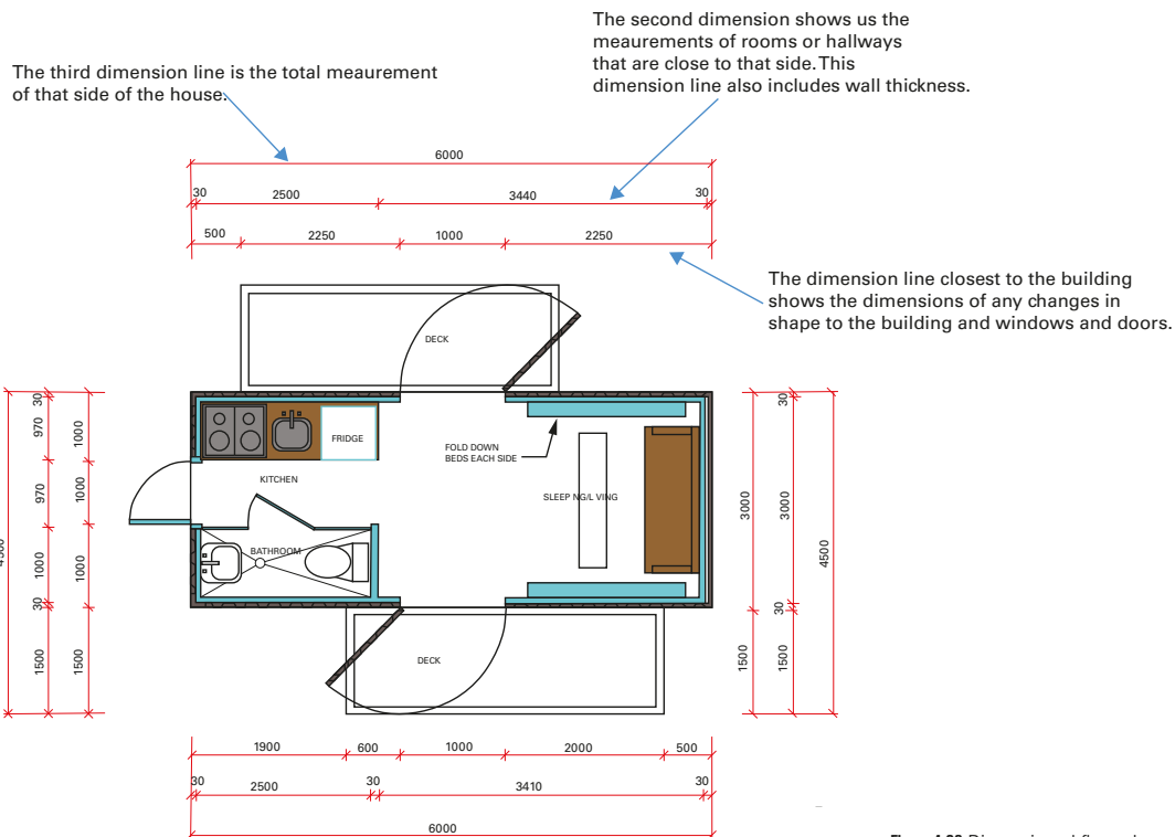
Figure 4.62 Dimensioned floor plan
