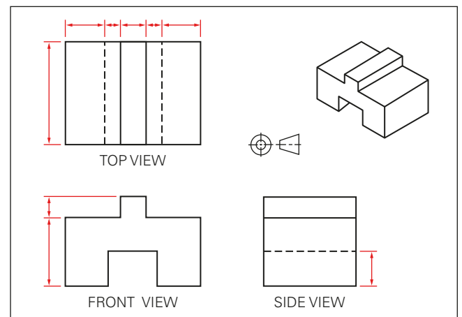
Figure 4.16 Placement of dimensions on the outside of the views
