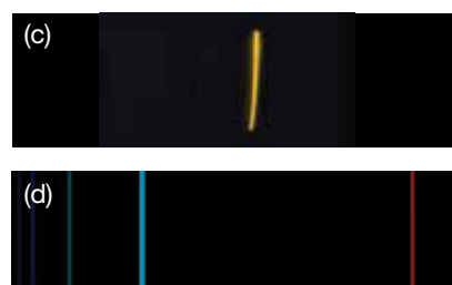
(a) Sodium vapour street light (whose spectrum is dominated by its yellow emission lines), (b) characteristic colour of sodium flame, (c) visible line spectrum of sodium atoms, and (d) visible line spectrum of hydrogen atoms
