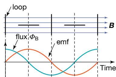
Flux-time graph
