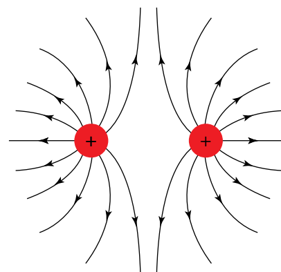
Fields around (a) a positive and negative charge of equal quantity, and (b) two positive charges of equal value. Close spacing of field lines indicates a strong field. Diverging lines indicate the field is weaker.
