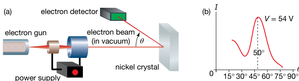
The Davisson and Germer experiment. (a) Electrons emitted from a heated filament are accelerated towards the crystal surface. The intensity of reflected electrons is recorded as the angle of the detector is changed. (b) Electron intensity as a function of angle
