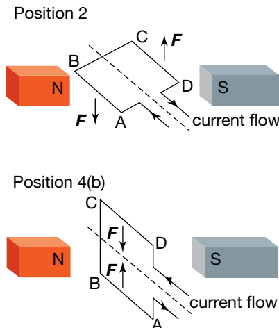
Force on a coil in a DC motor
