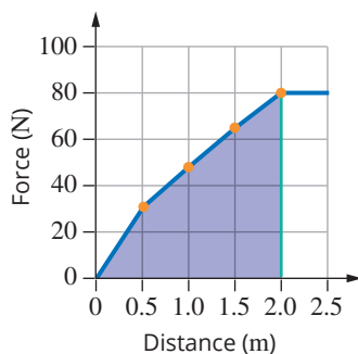
Force vs distance stretched of rubber tubing
