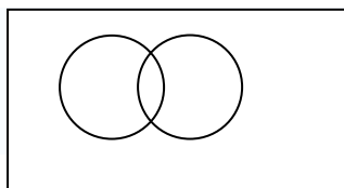
OVERLAPPING SETS
