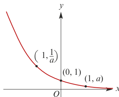
Graph of f(x) = a^x for 0 < a < 1
