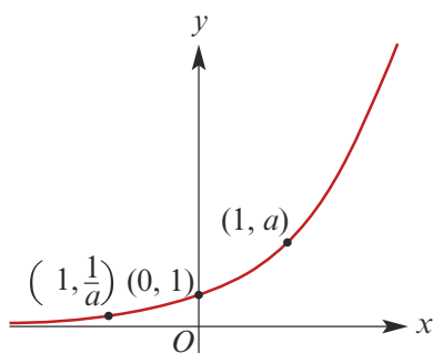
Graph of f(x) = a^x for a > 1
