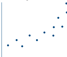
Scatterplot A
