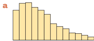
Age distribution in a country
