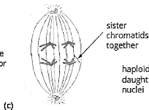
Anaphase I
