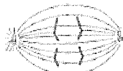
Anaphase II
