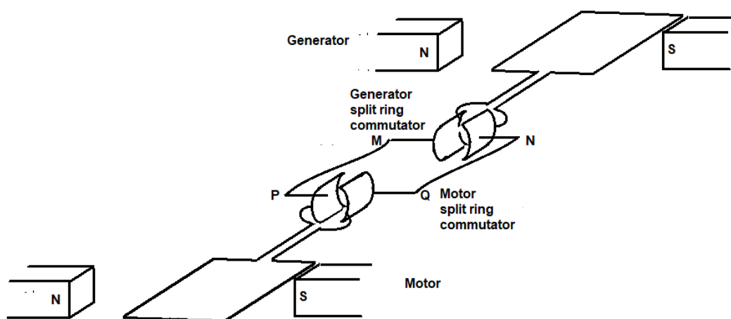
Figure 4 The generator and motor are on separate axles. The devices share an electrical connection.
