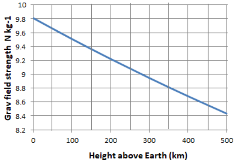
Figure 4 The graph shows the variation in the Earth's gravitational field at these heights.
