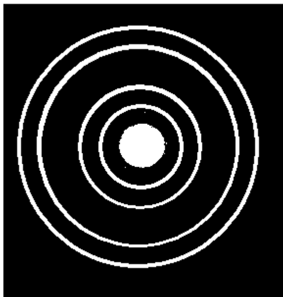
Figure 20 The diffraction ring produced by the 15.6 keV photons
