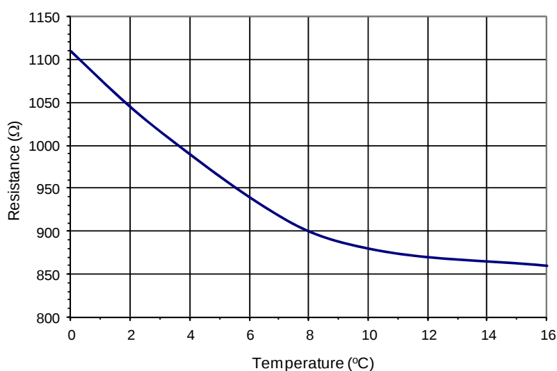
Thermistor Resistance vs Temperature
