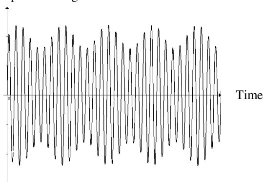
B. Amplitude of light wave
