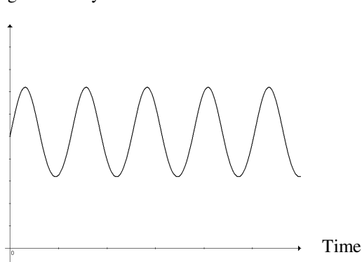
D. Light intensity
