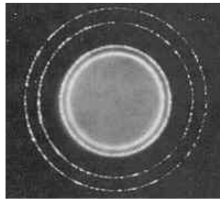
Photo 1: X-ray scattering
