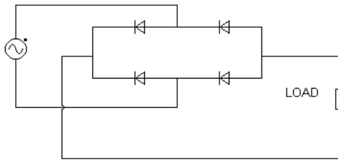
CIRCUIT C
