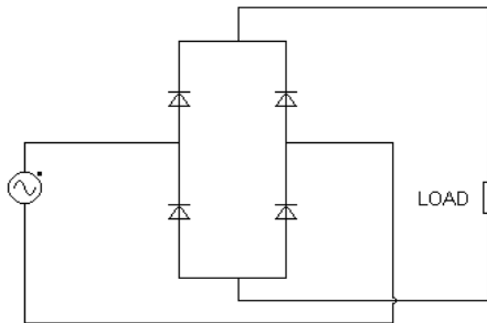
CIRCUIT C
