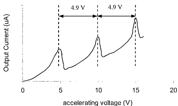
Franck Hertz Experiment
