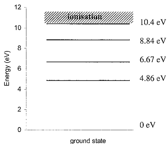
Energy levels for Hg
