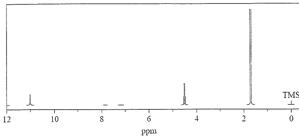
^1\text{H} NMR spectrum
