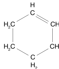
Figure 4.1 Cyclohexene ( C_6H_{10} ).
