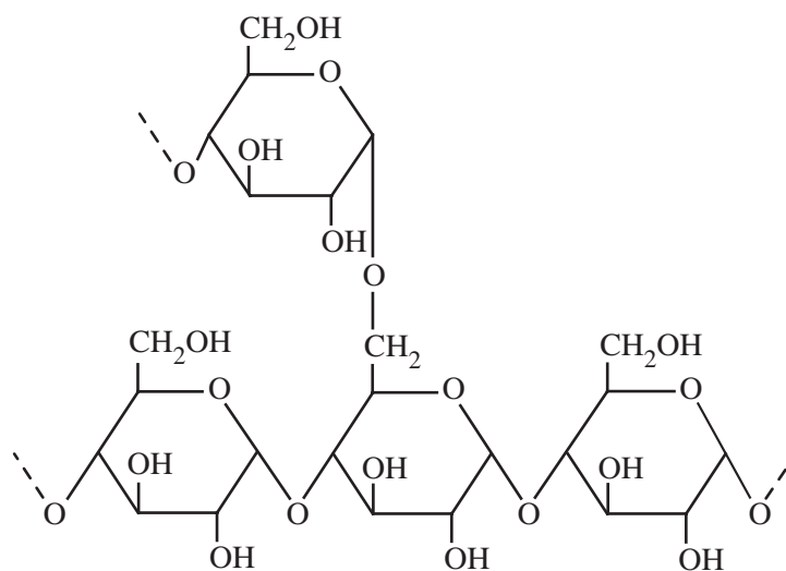
amylopectin (starch)
