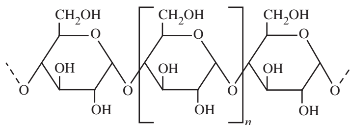
amylose (starch)
