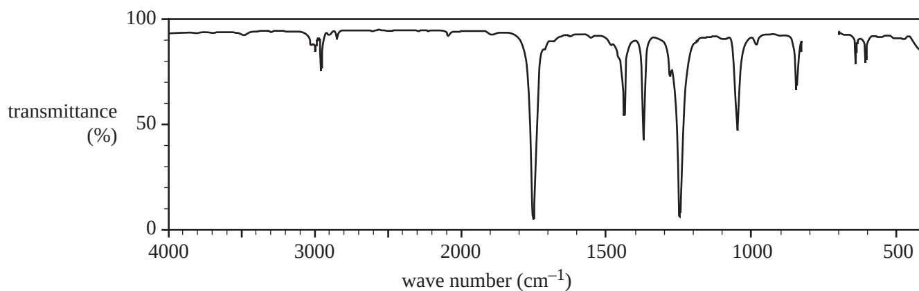
Infra-red spectrum
