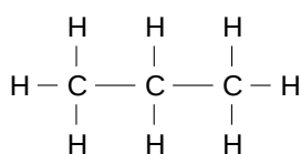
A propane
