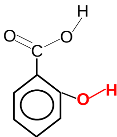
Salicylic acid
