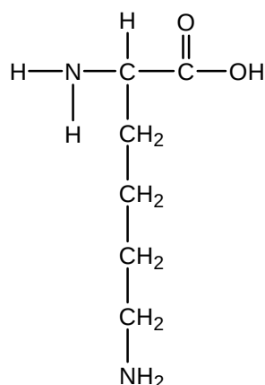
Lysine
