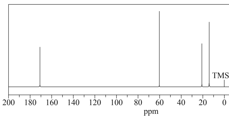
^{13}\text{C} NMR spectrum
