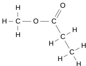
methyl propanoate*
