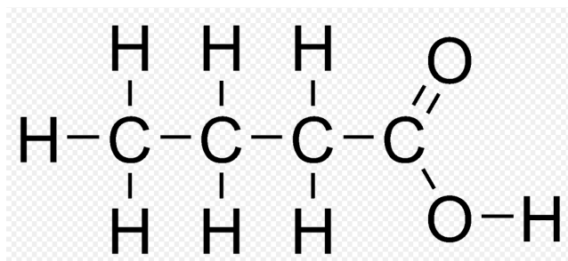
butanoic acid
