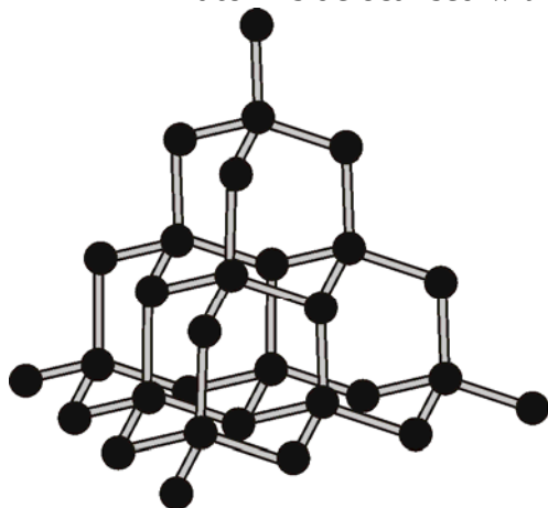
Diamond
