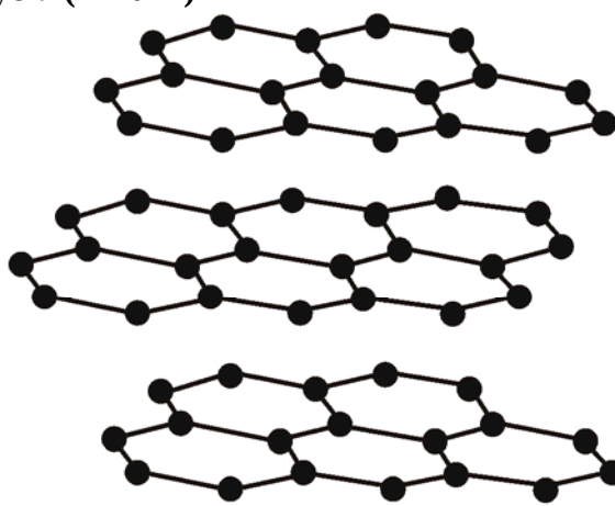
Graphite
