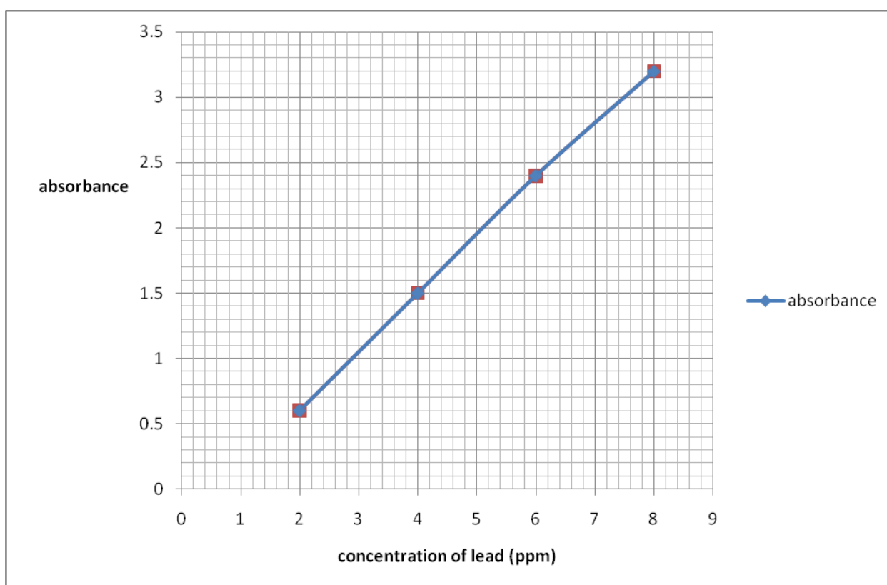
Calibration graph
