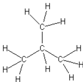
2-methyl propane
