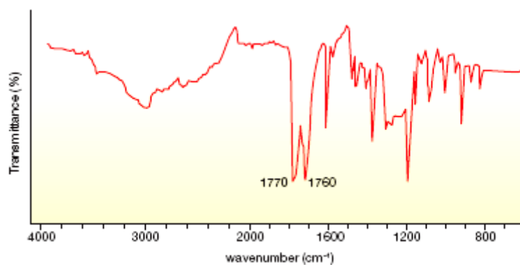
Infra-Red Spectrum of Acetylsalicylic Acid
