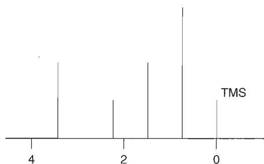
low resolution ^1\text{H} NMR spectrum
