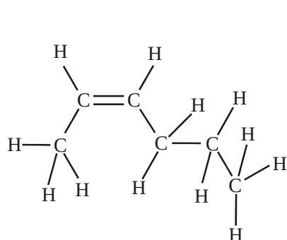
hex-2-ene
