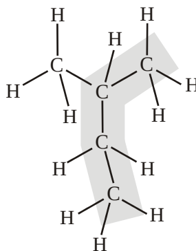
2-methylbutane
