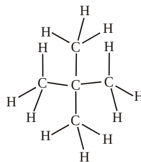
2,2-dimethylpropane
