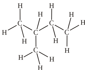
2-methylbutane
