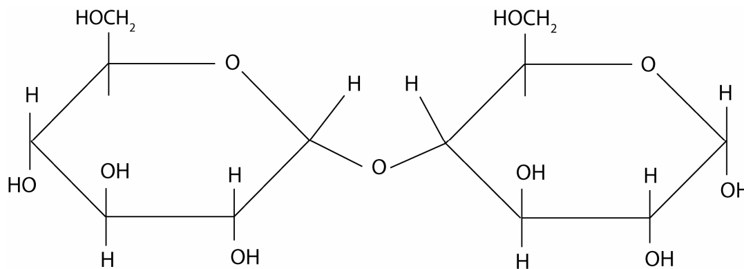
Molecule C
