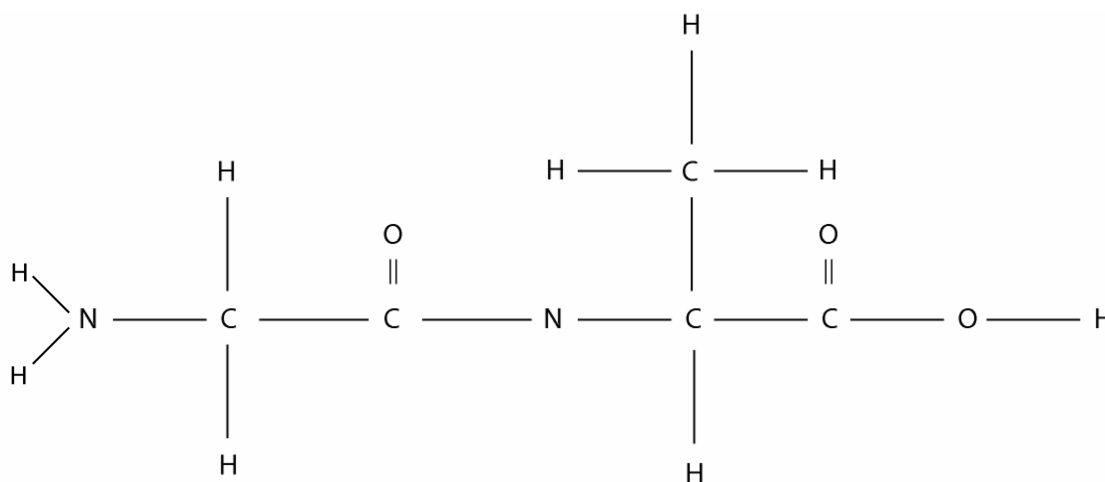
Molecule B
