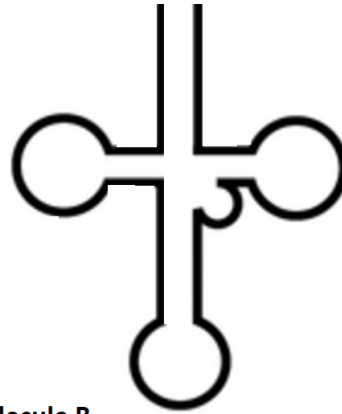
Molecule B
