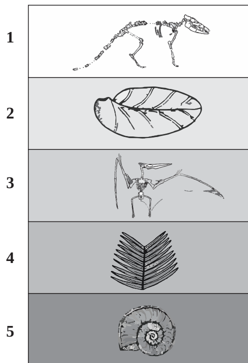
Figure 1: A segment of sedimentary rocks containing fossils
