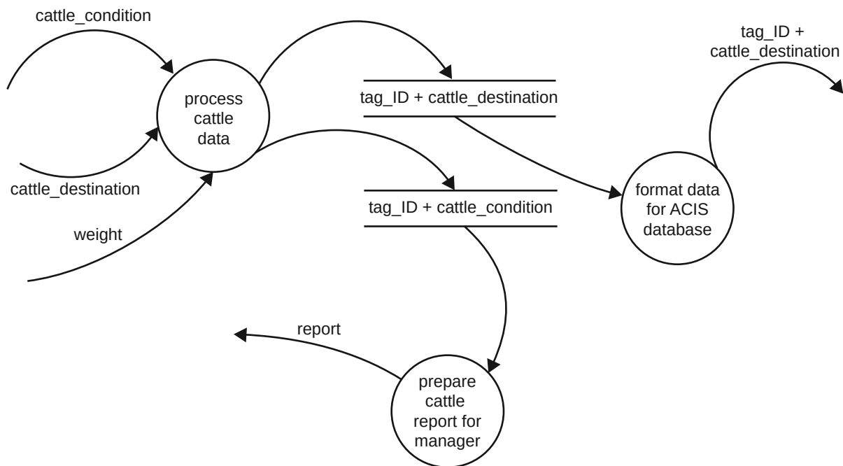
Diagram 3: Data flow diagram (DFD)
